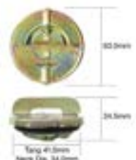
Petrol Cap Non Locking TFNL207
