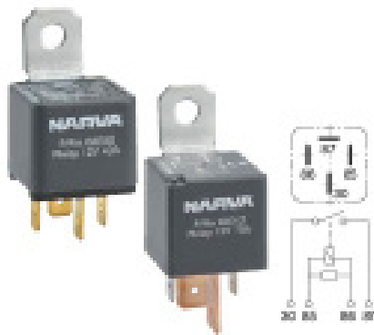
Fig. 2: 4 pin relay and variants over 50 amp have a 9.5mm pin (86) and 87 terminals
